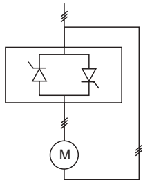
Connection in the motor delta connection
